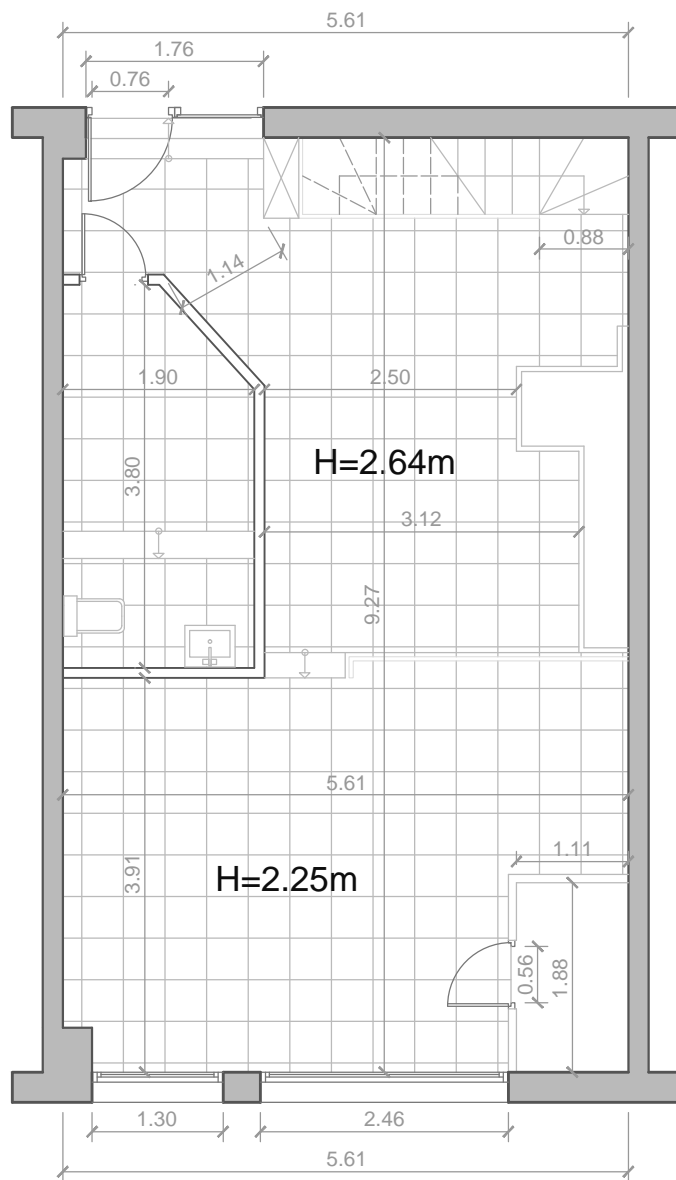
LEHEN OINA A_{\text{erabilgarria}} = 49.38 \text{ m}^2 A_{\text{eraikia}} = 57.64 \text{ m}^2
